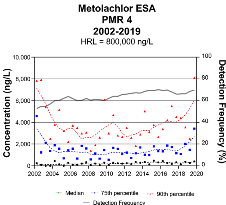
Figure 6. Metolachlor ESA, a Metolachlor degradate, groundwater sample analysis results over time for the Central Sands monitoring network (PMR 4).
